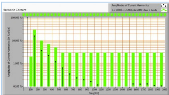
Harmonics in the current waveform and checked against IEC61000-3-2:2006 and A2:2009
