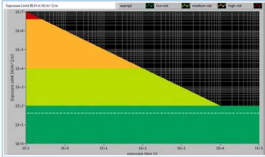
The level of blue light of this lamp related to the exposure limit and the different classification areas.
