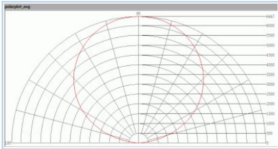
The radiation pattern of the light bulb.
