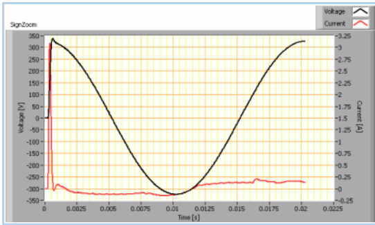
First cycle of the maximum inrush current
