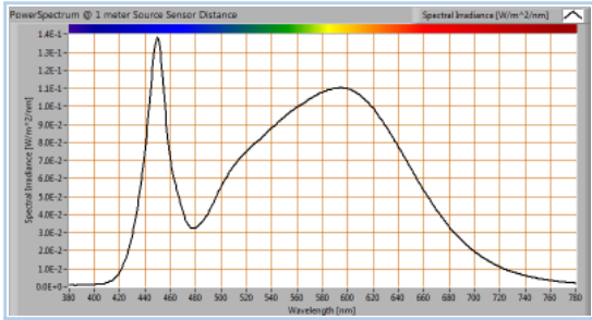
The spectral power distribution of this light bulb, energies on y-axis valid at 1 m distance.
