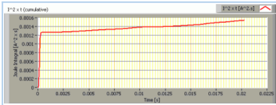
The energy I^2 t during the first 10 ms of the first current cycle
