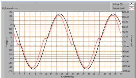
Voltage across and current through the lightbulb
